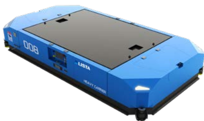
LISTA Heavy Carrier for transporting large weights of up to 30 t
